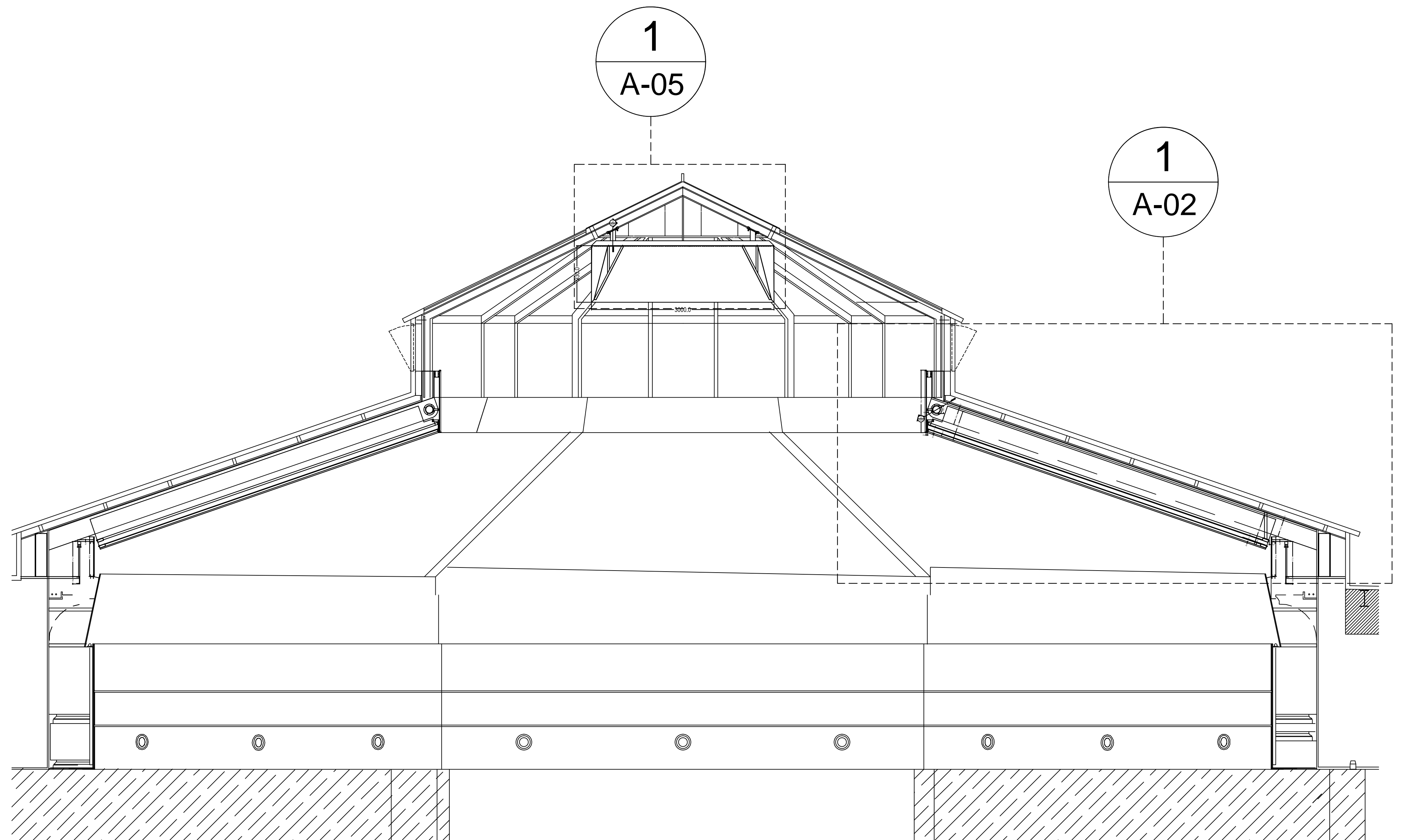
2 SECTION
