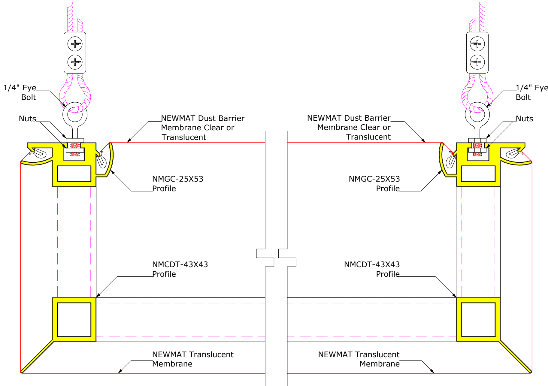
NMCDT-43X43 Profile with 2 layers of membranes detail CCT-2LS
