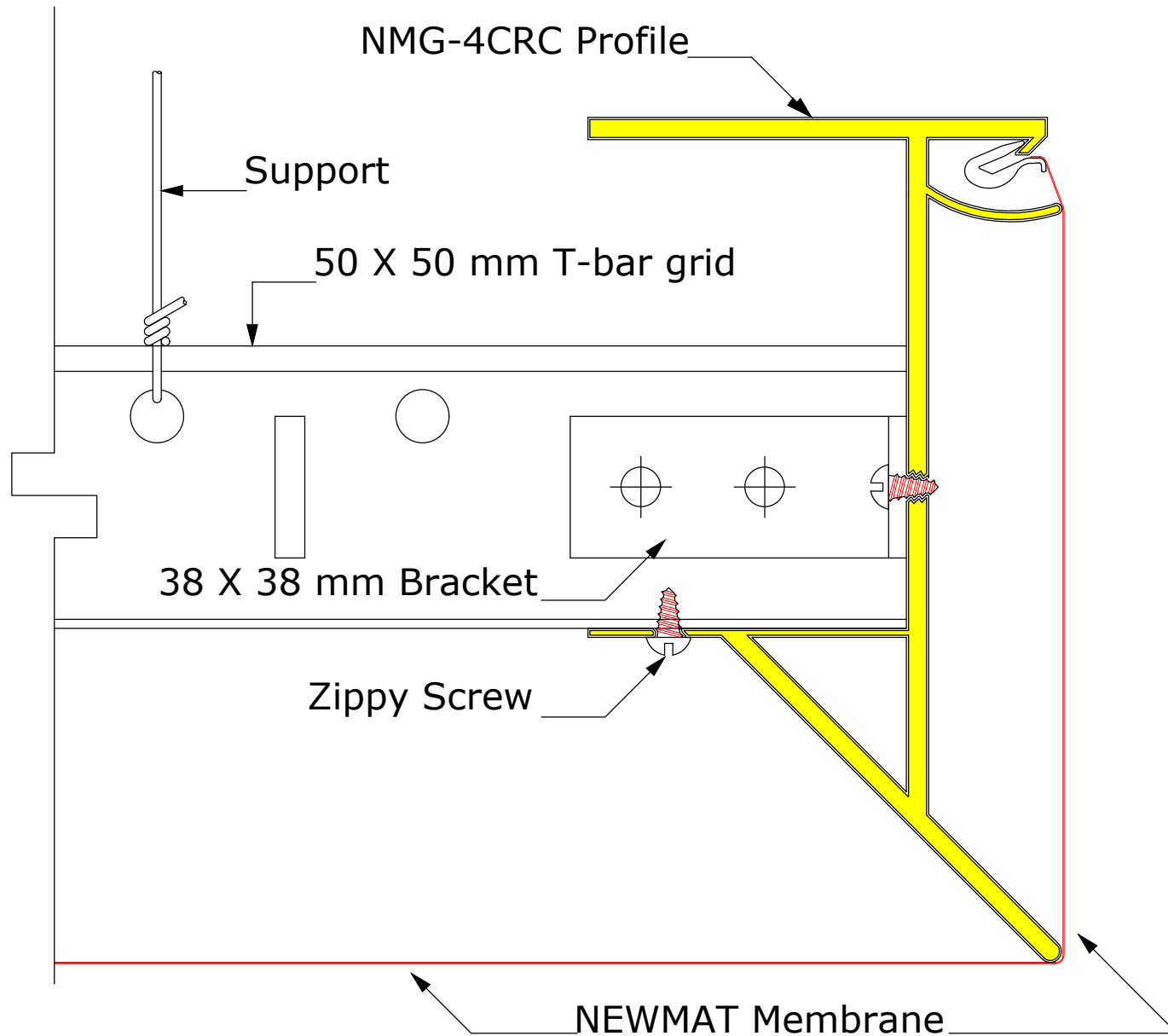
Ceiling Cloud with NMG-4CRC Profile and 600X600 mm T Bar grid Detail CRC-24
