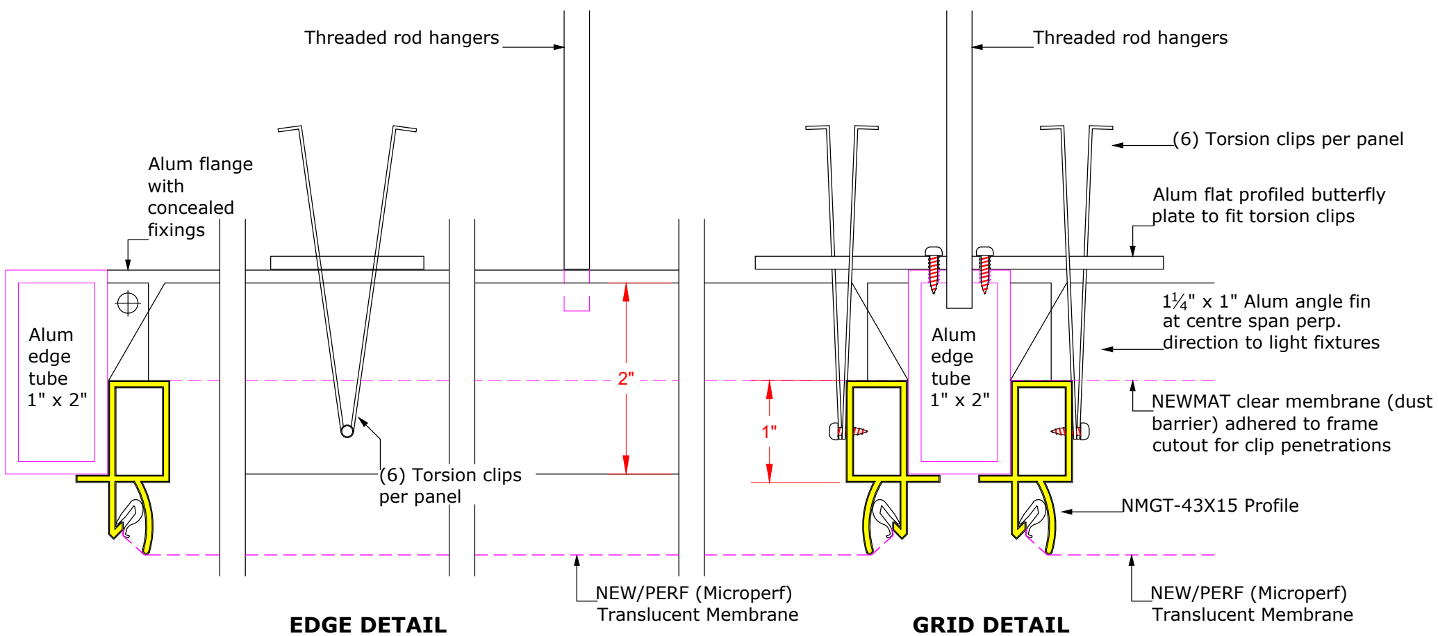
Ceiling Cloud with Acoustical & Translucent Accessible Panels - Detail CCA-TAP
