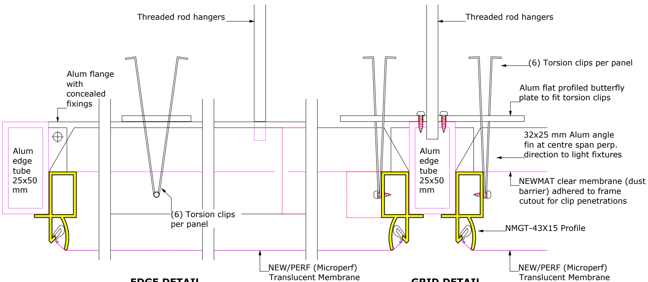
Ceiling Cloud with Acoustical & Translucent Accessible Panels - Detail CCA-TAP
