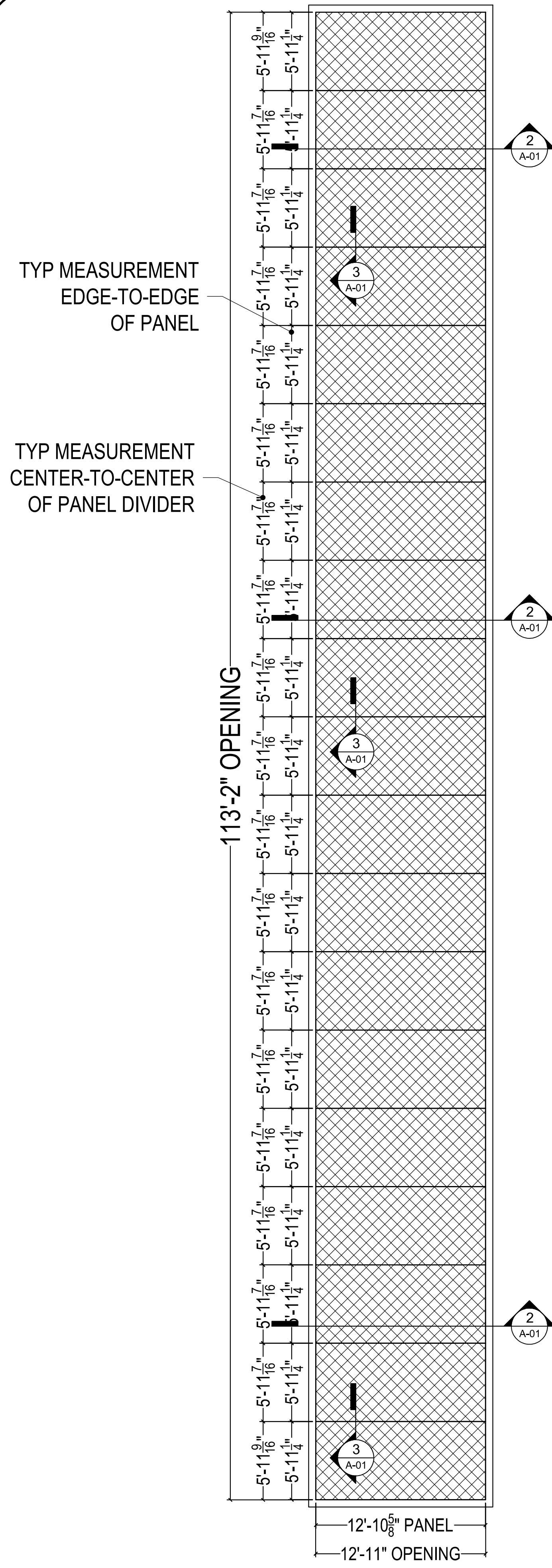
1 PARTIAL RCP @ SECOND FLOOR CAFETERIA SCALE: NTS
