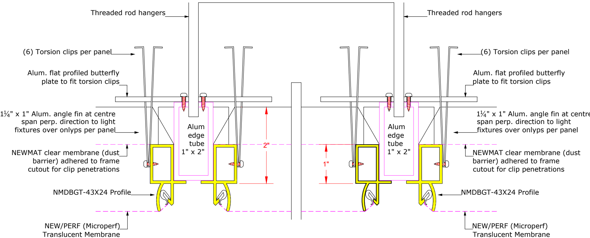
Translucent Panels on Torsion Clips - Detail ATP-1
